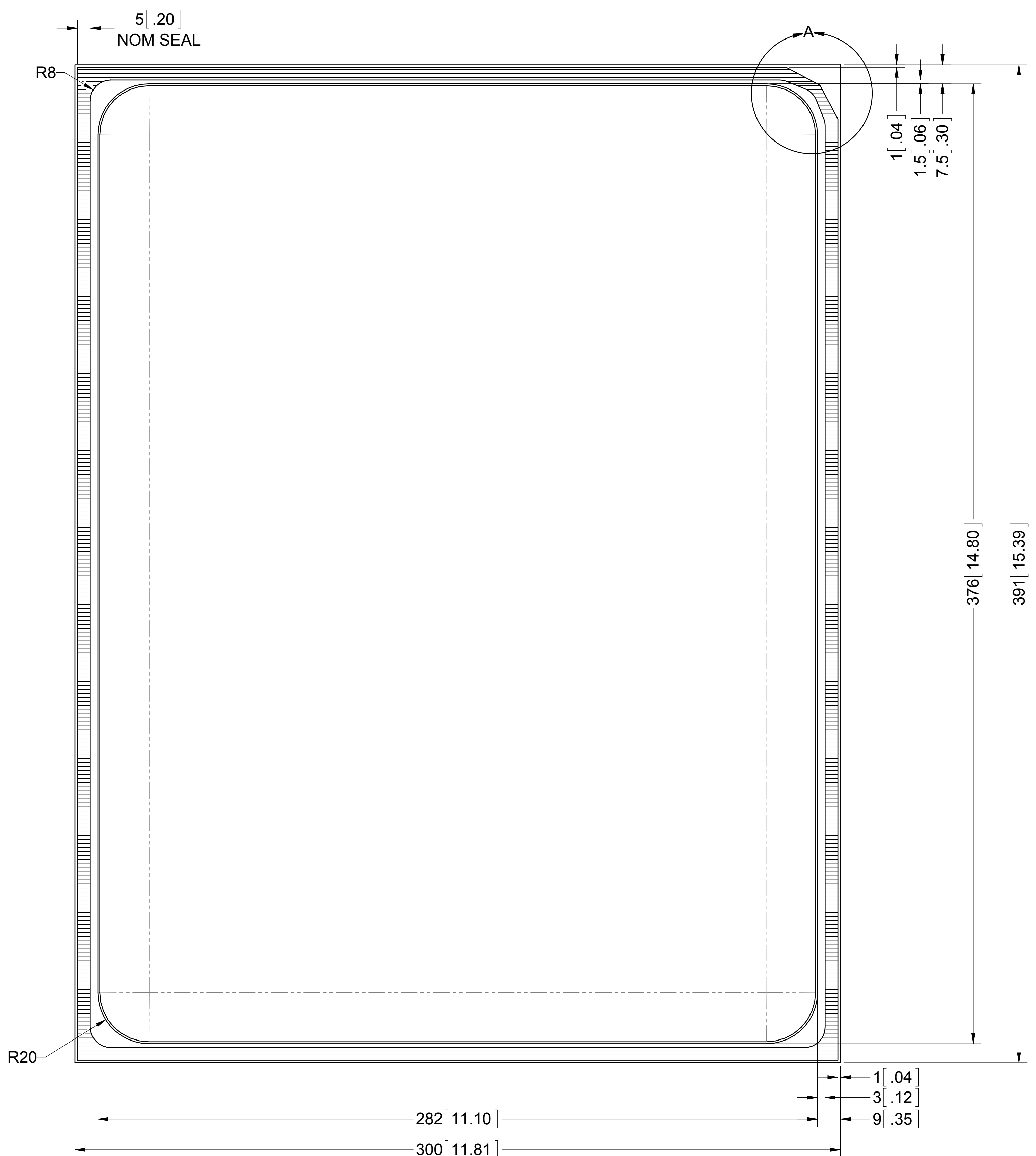
TYPICAL SINGLE PACKAGE TOP VIEW
